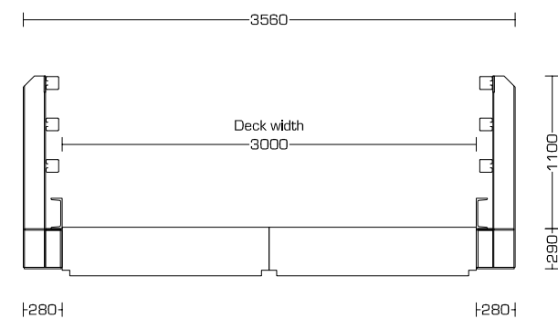
Cross view JSK 300 series - 300mm Construction height [1-50]
