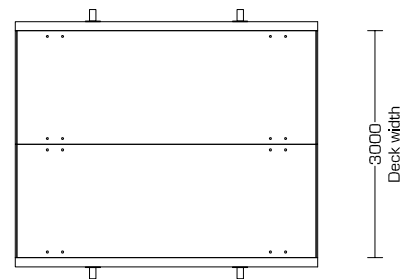
Top view JSK 300 series - 3,00m Deck width [1-100]
