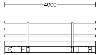
Side view JSK 300 series - 4,00m Free span [1-100]
